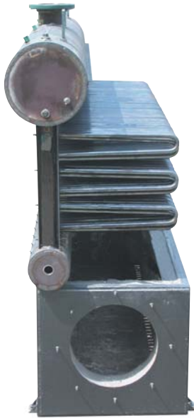
Steam Boiler
