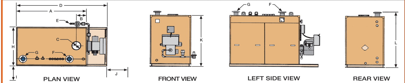
HOT WATER HEATING BOILER DIMENSIONS in inches (cm)
