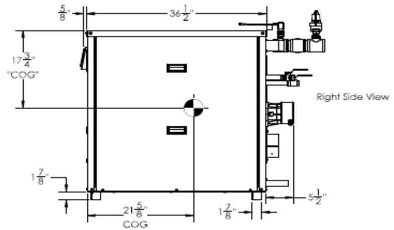
400-500 Boiler Dimensional
